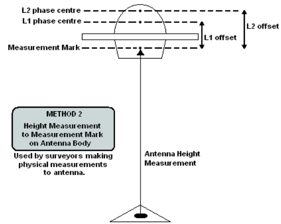
Figure 7: Antenna Measurements
