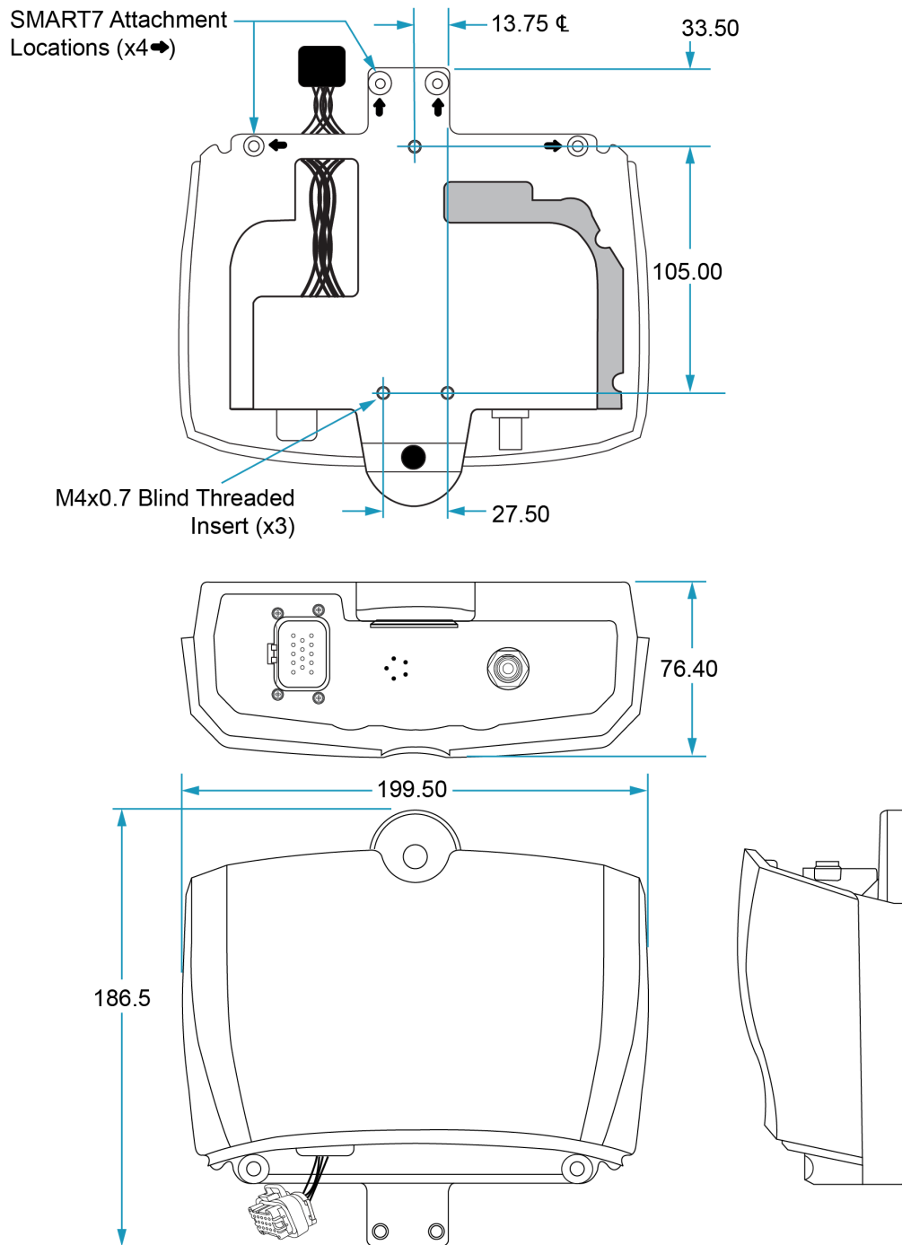
Figure 10: RELAY7 Dimensions
