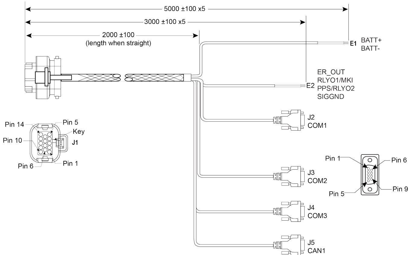
Figure 10: SMART Antennas Interface Cable
