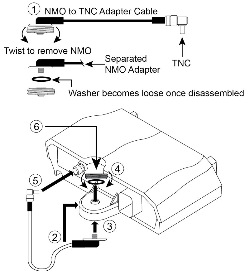
Figure 6: RELAY7 Antenna Mounting
