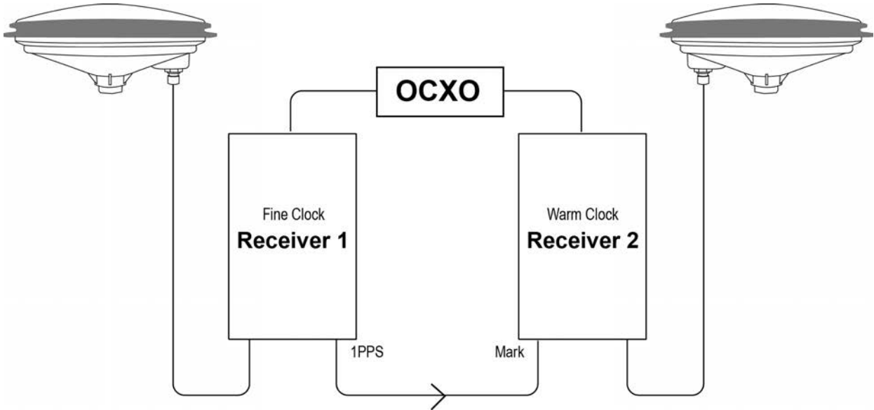
Figure 3: ADJUST1PPS Connections
