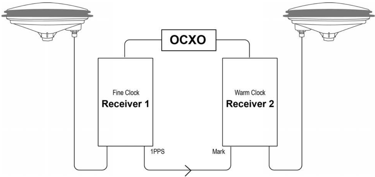
Figure 3: ADJUST1PPS Connections
