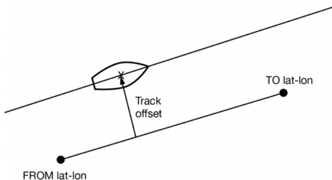
Figure 9: Illustration of SETNAV Parameters
