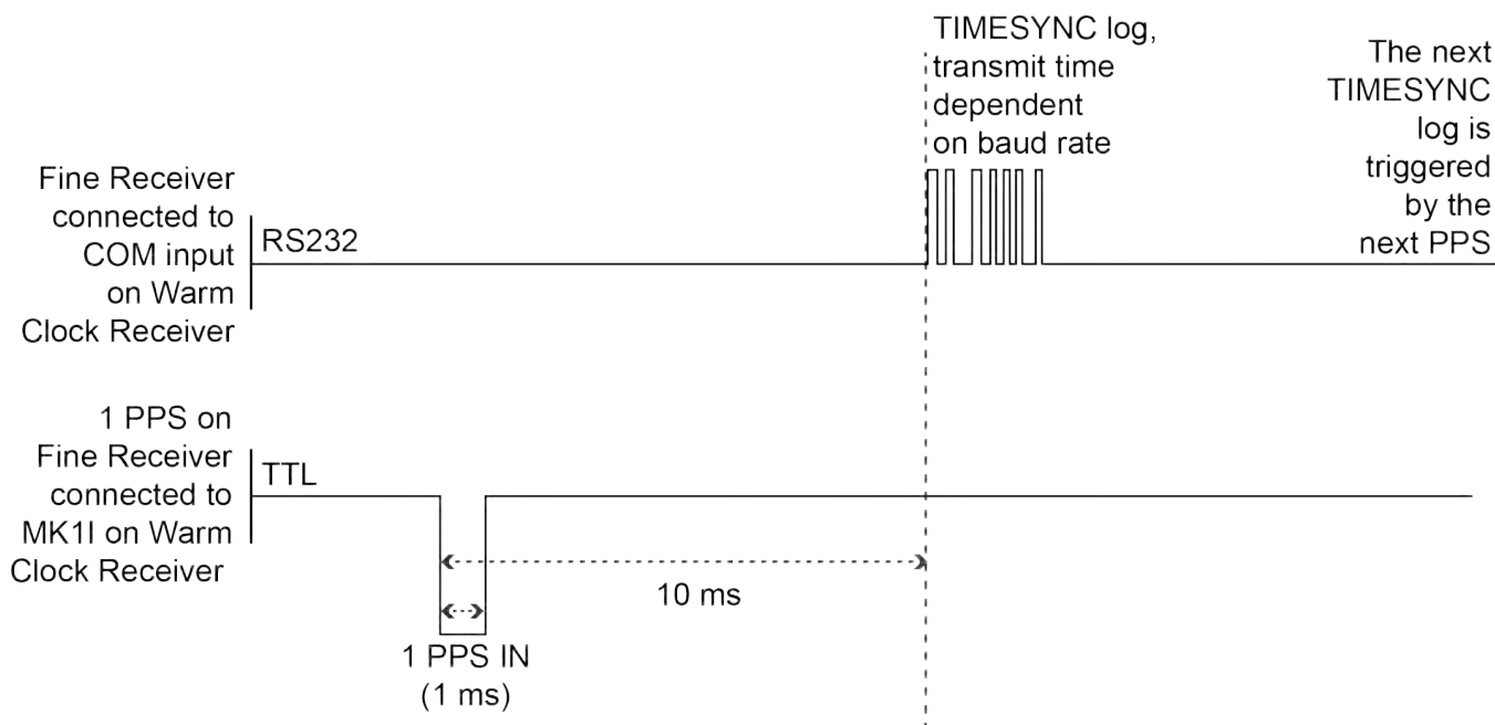
Figure 2: 1PPS Alignment
