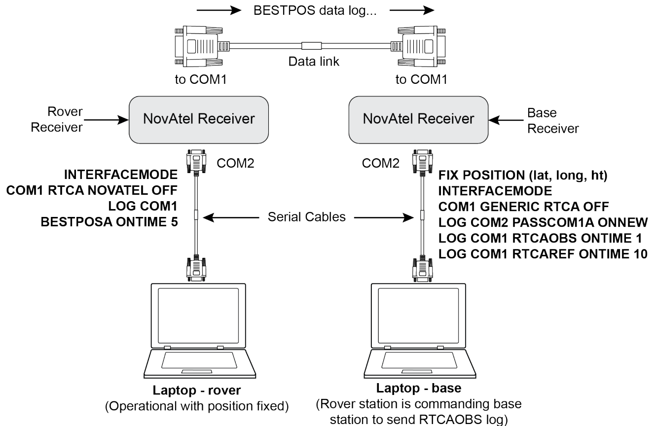
Figure 8: Pass Through Log Data
