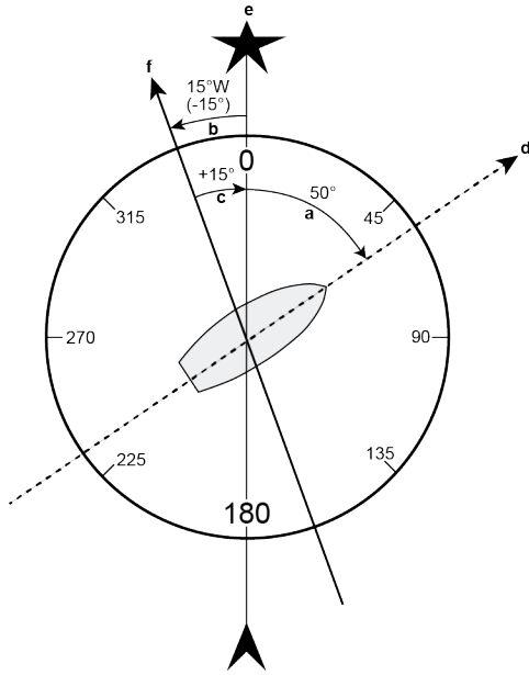
Figure 3: Illustration of Magnetic Variation and Correction
