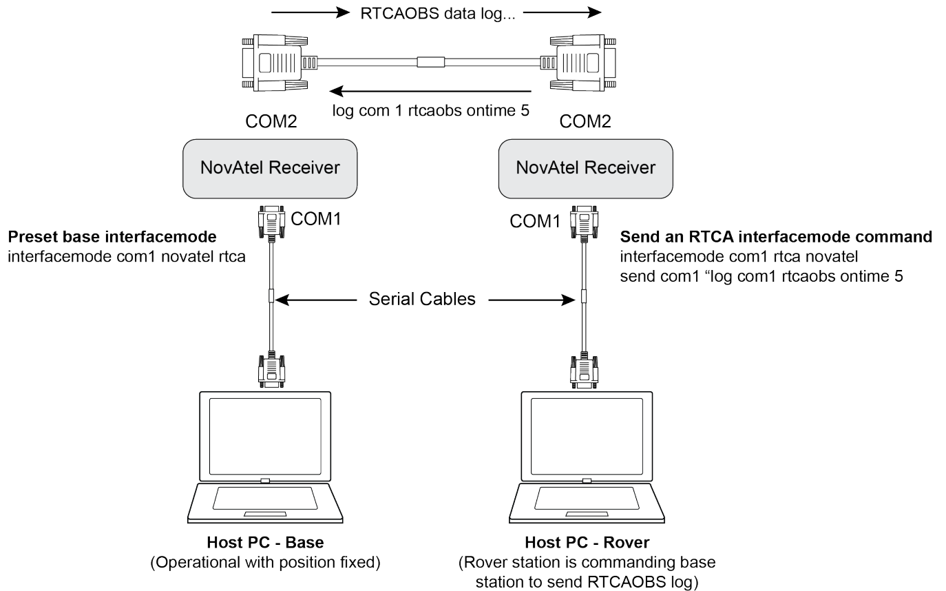
Figure 5: Using the SEND Command
