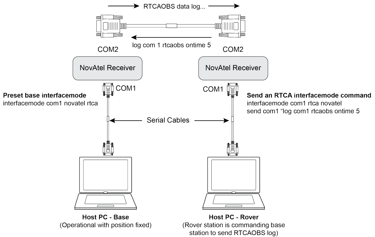
Figure 4: Using the SEND Command
