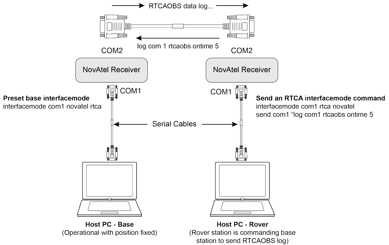
Figure 4: Using the SEND Command
